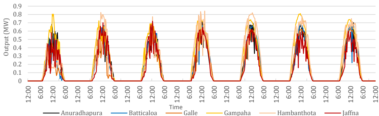
A5.6 Extract of Solar PV Production based on actual measurement data (15 minute)
