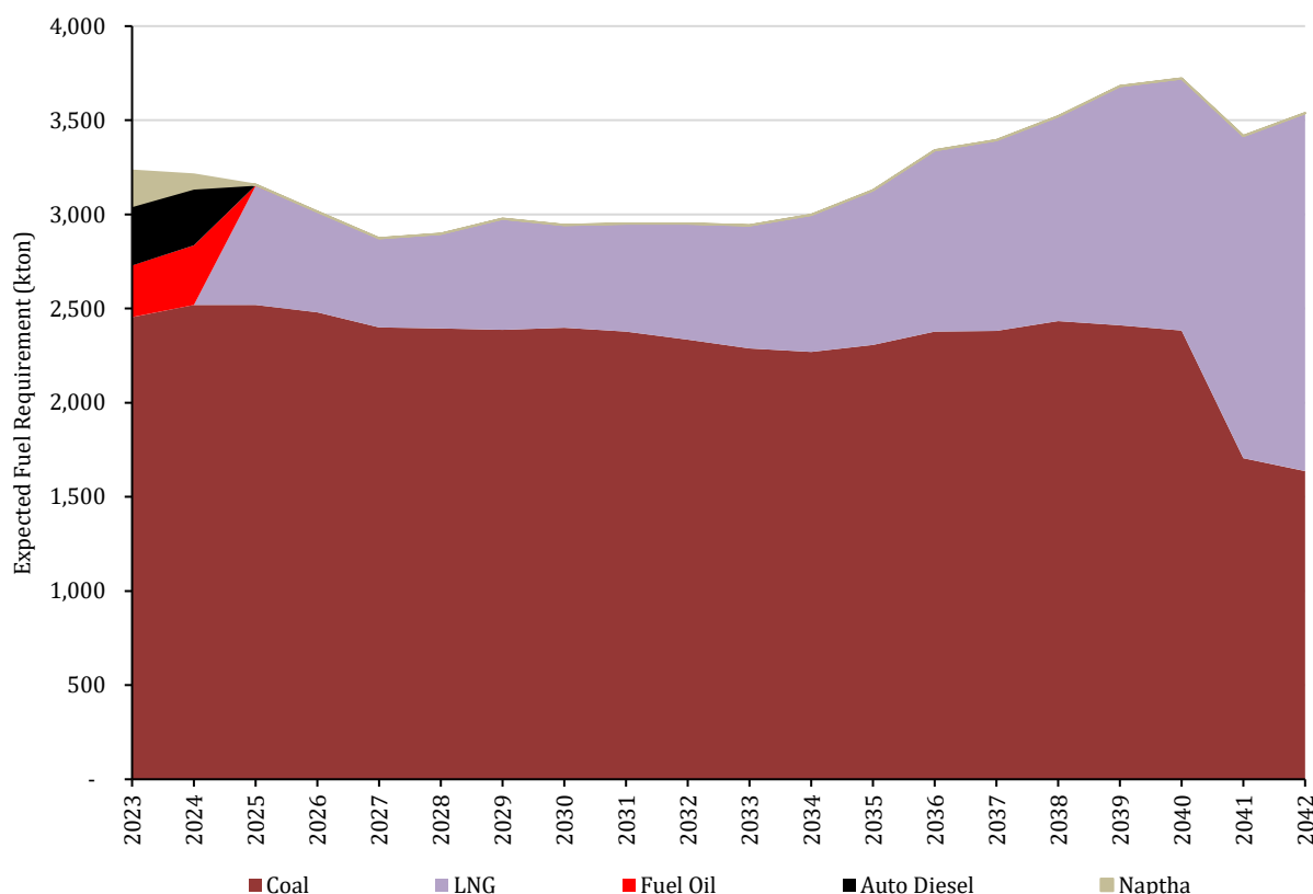
Figure 8.8 - Fuel Requirement of Base Case
