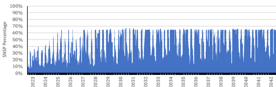
Figure 9.2 – Distribution of SNSP from 2023-2042
