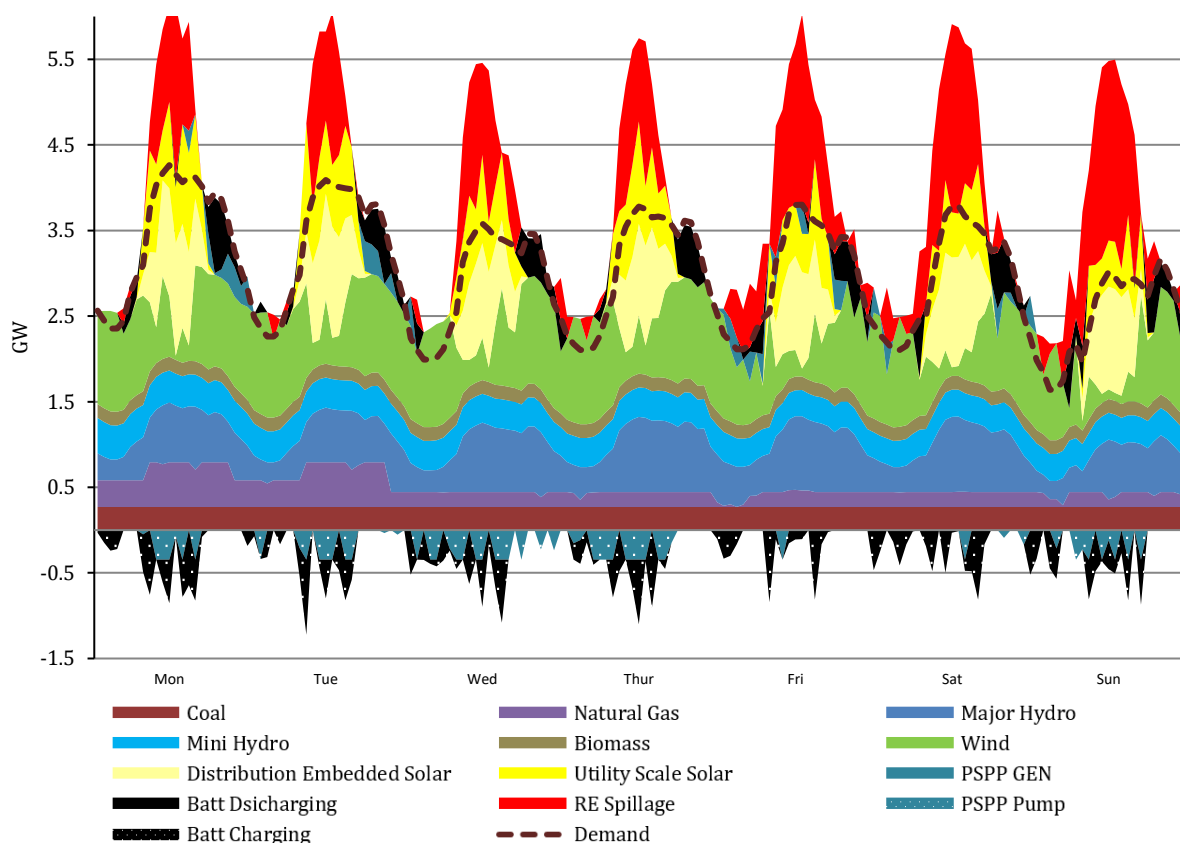
Figure 9.6 – Sample Weekly Dispatch During High Wind Season – September 2030
