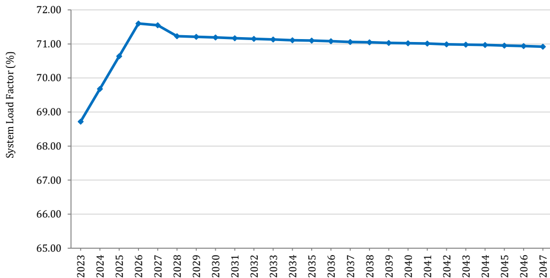
Figure 3.7 – System Load Factor Forecast 2023-2047
