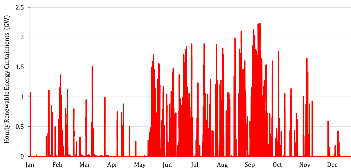
Figure 9.10 - Annual Curtailment Pattern of Year 2030
