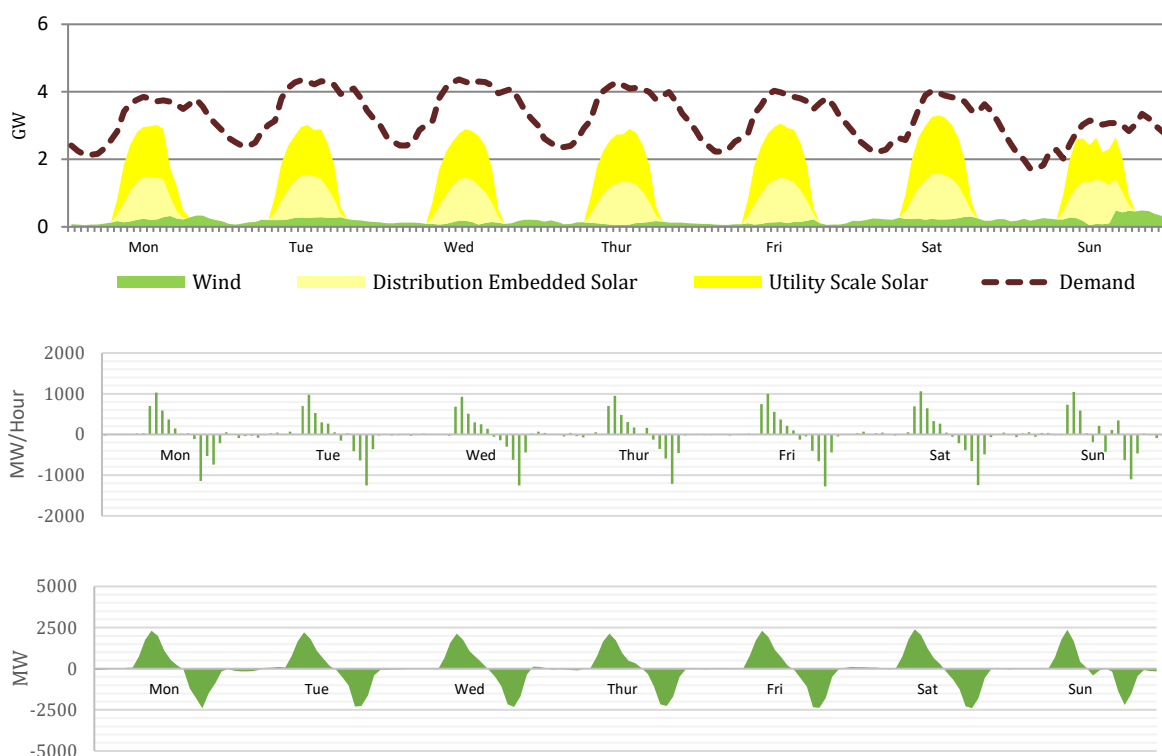
Figure 9.15–Generation, Hourly Ramping & Daily Ramping of VRE - Dry Season Week 2030
