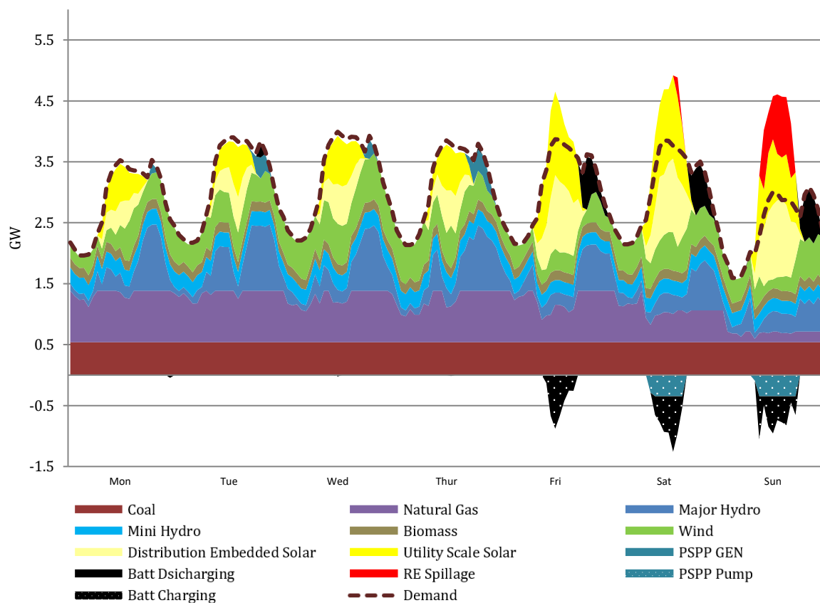
Figure 9.7 – Sample Weekly Dispatch During Wet Season – December 2030
