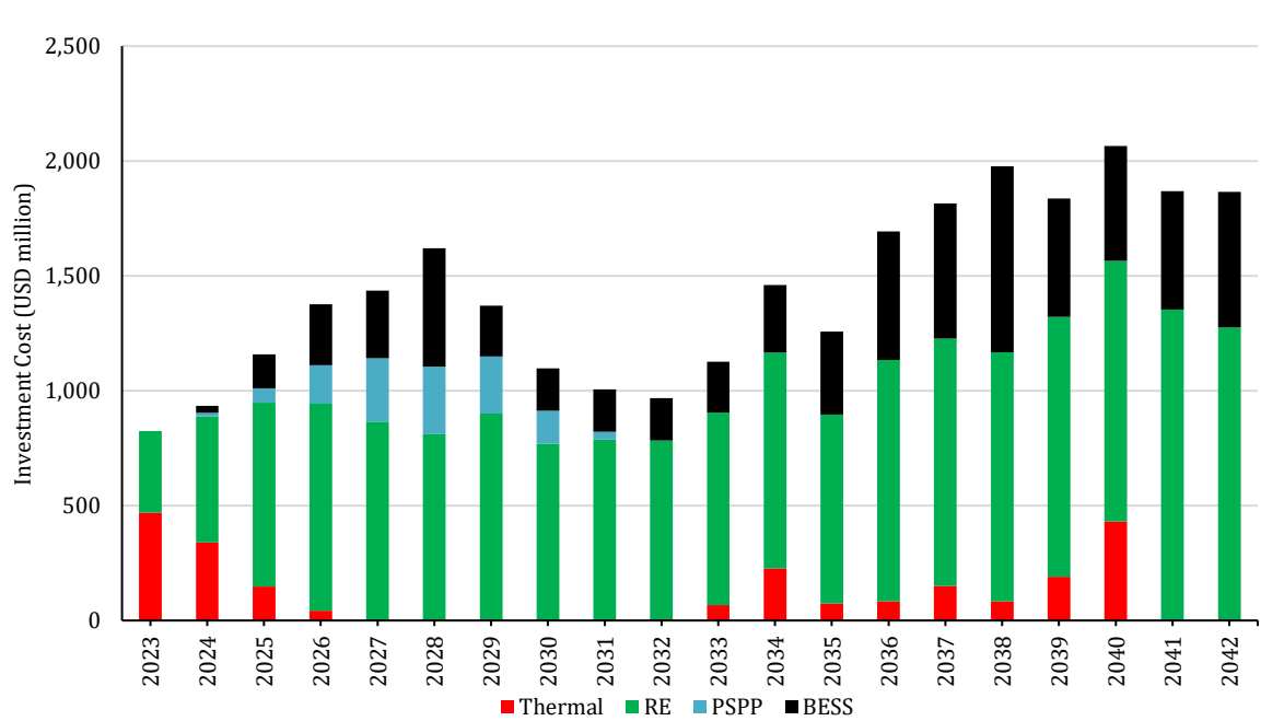
Figure 13.4 - Technology Wise Investment Plan for Base Case 2023 -2042
