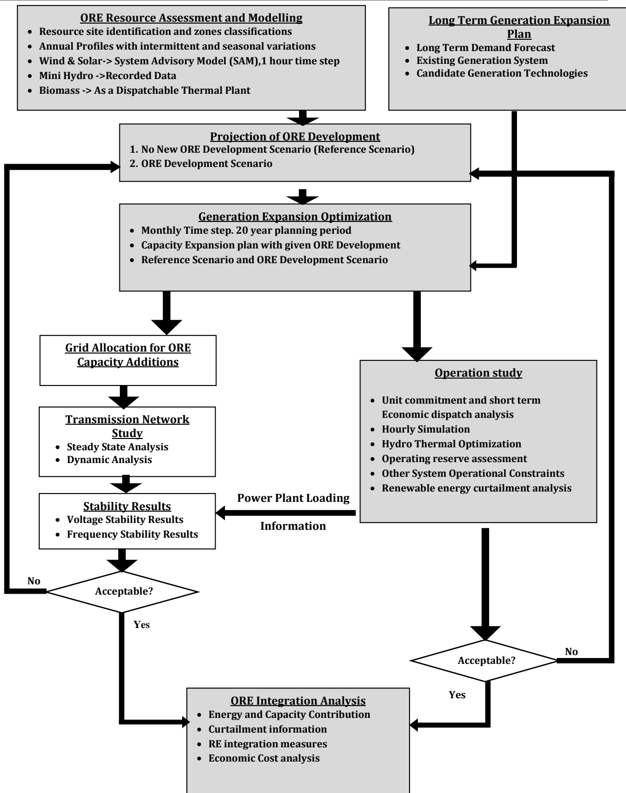
A5.1 Outline of the study methodology of renewable energy integration study 2023-2032
