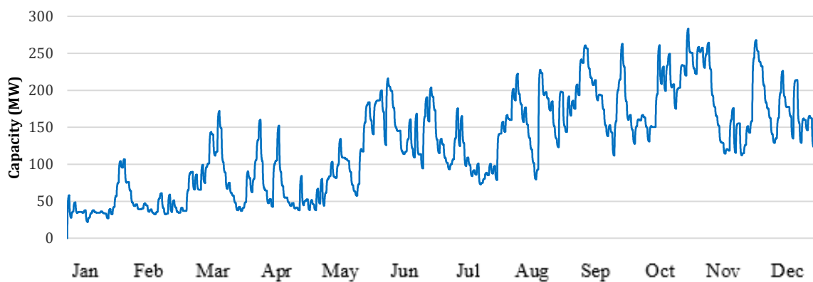
A5.7 Modelled production profile of Mini-hydro resource
