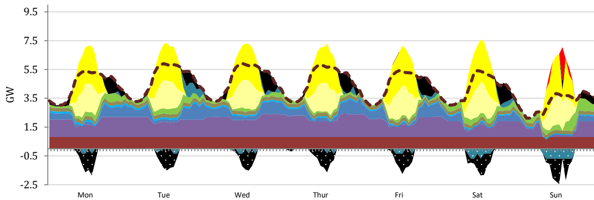
Dispatch Profile of Dry Season in Year 2036
