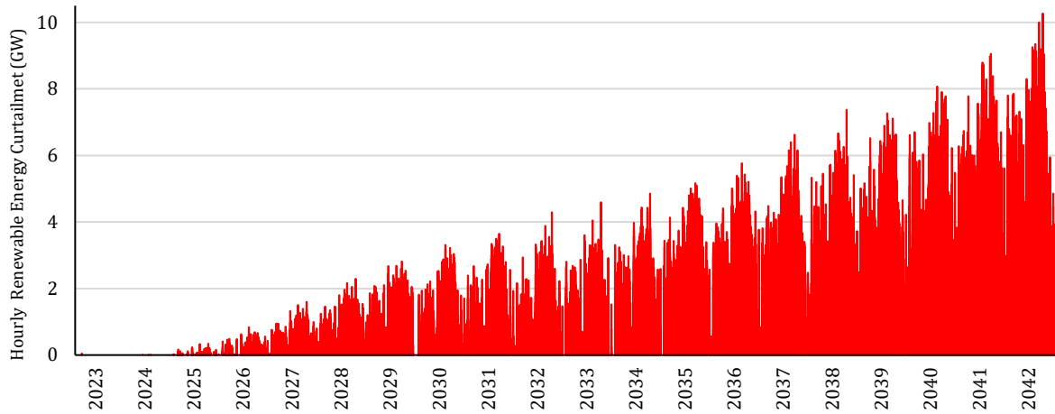
Figure 9.8 – Renewable Energy Curtailments 2023-2042
