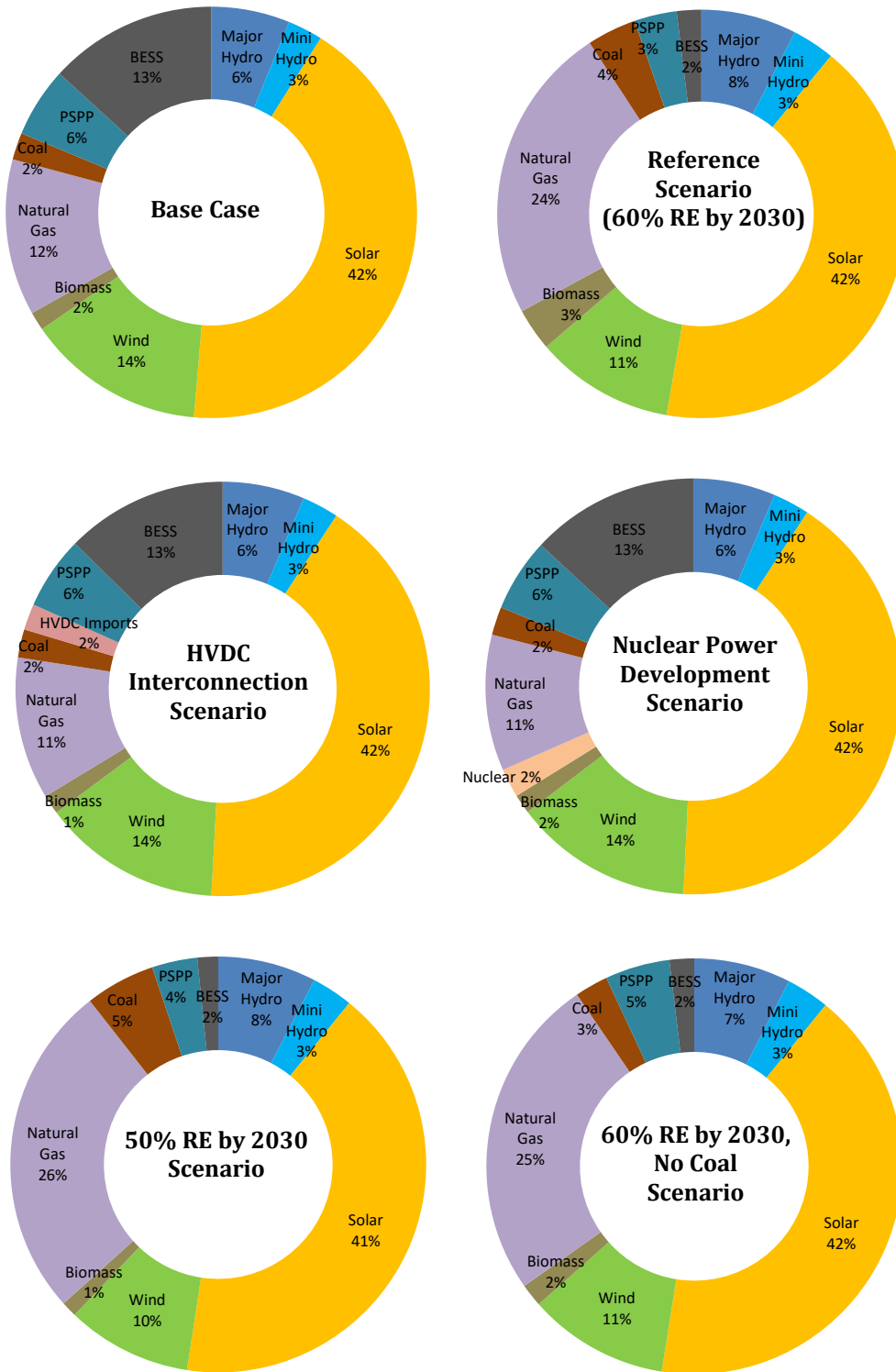
Figure 10.5 – Installed Capacity Share Comparison in 2042
