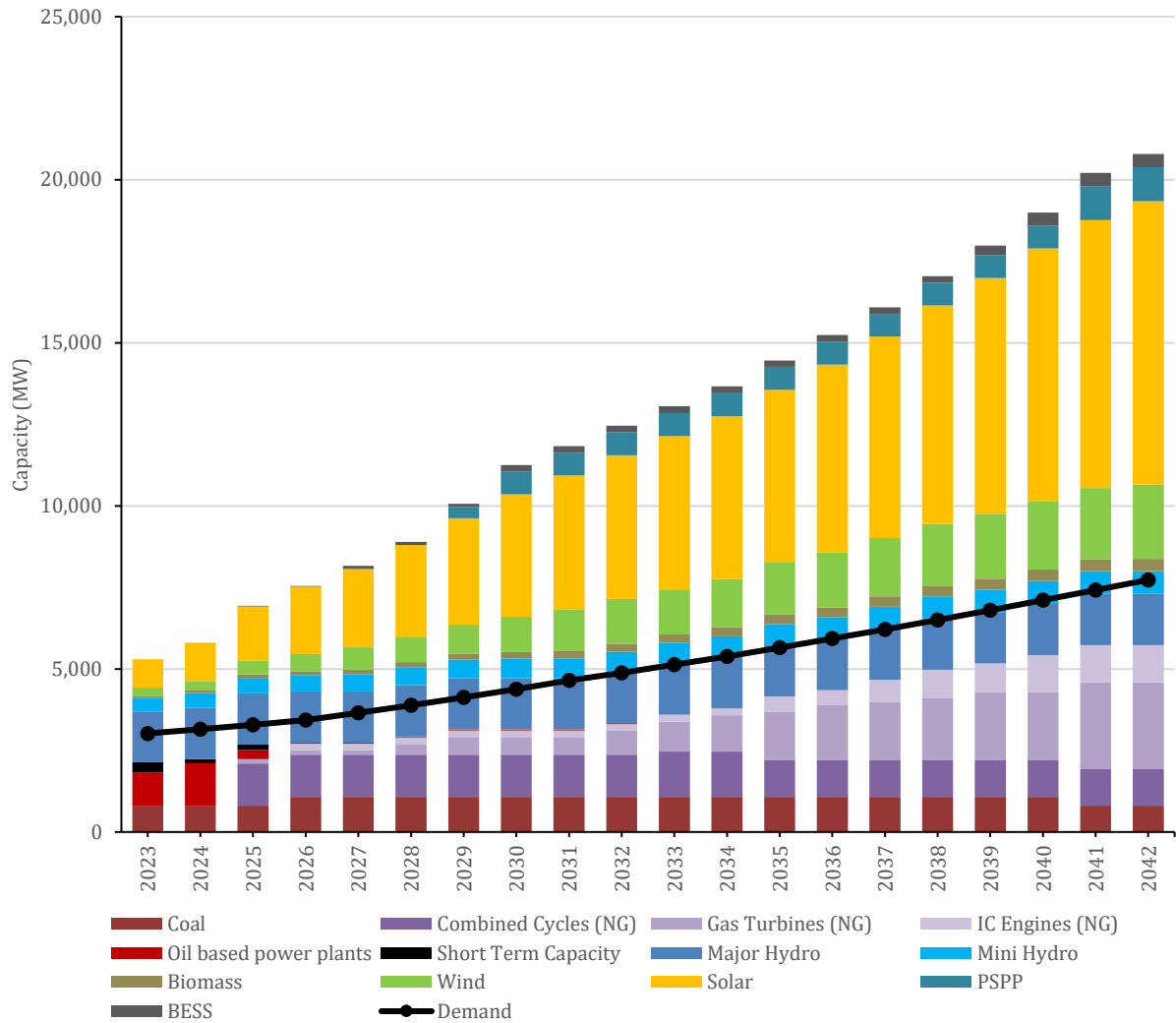
Figure 7.1 - Cumulative Capacity by Plant Type in Reference Case
