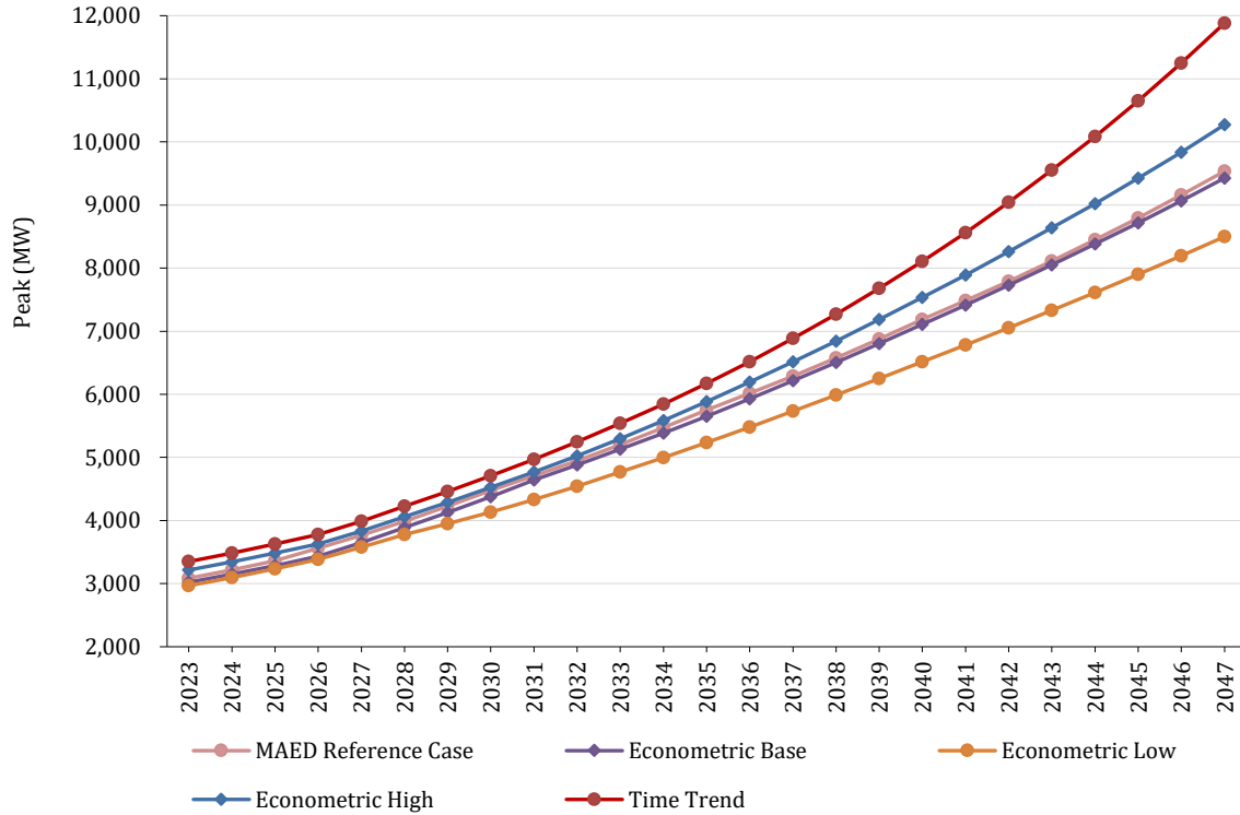
Figure 3.11–Peak Demand Forecast Comparison - Econometric, Long Term Time Trend and MAED Model
