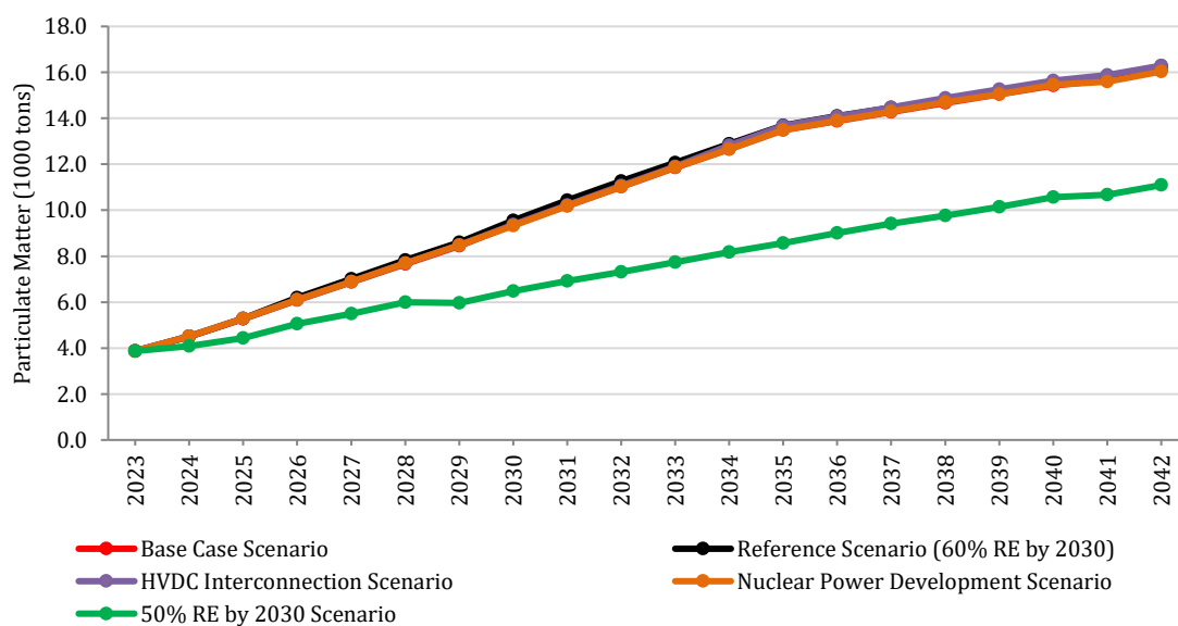
Figure 11.9 - Particulate Matter Emissions
