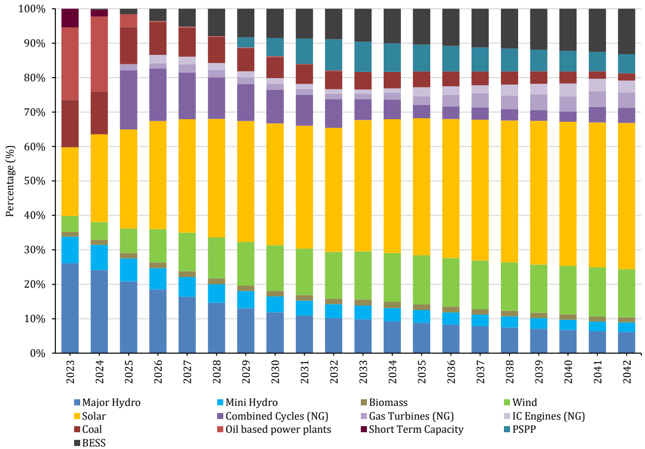
Figure 8.2 – Capacity Mix over Next 20 Years in Base Case
