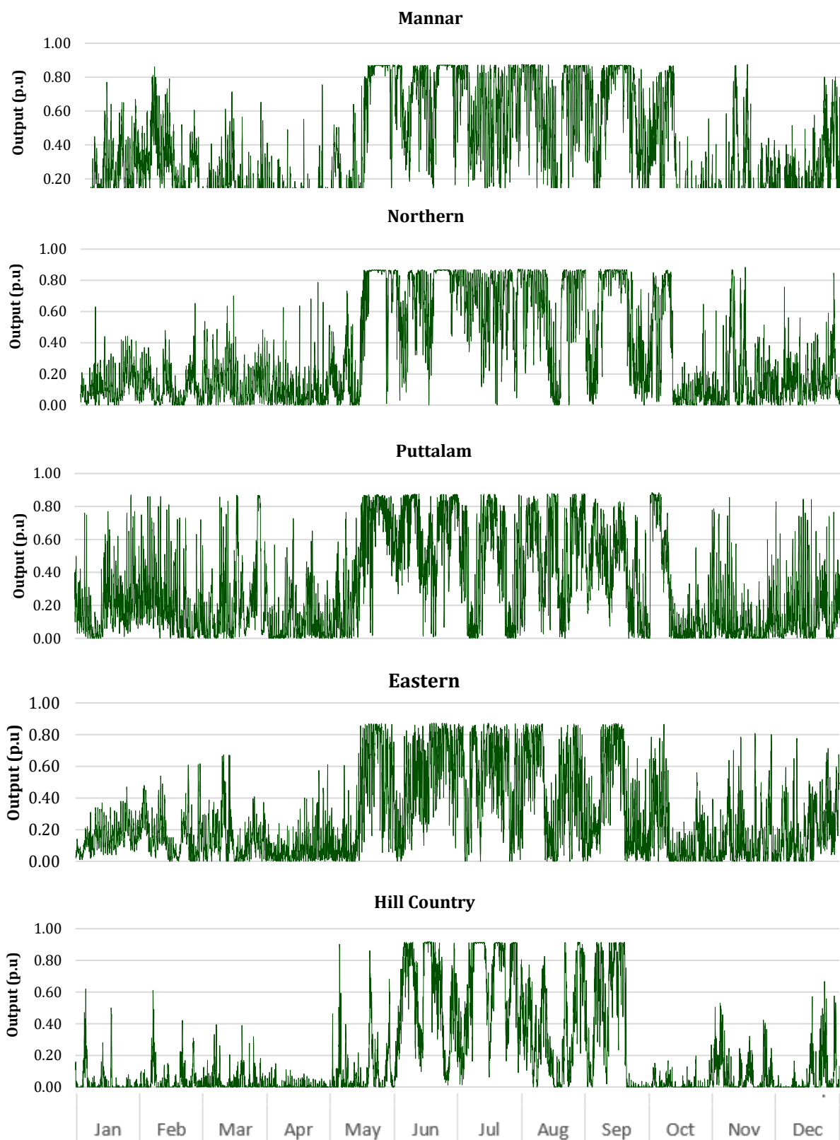
A5.5 Annual variation of wind power production in different regions (Based on 10 min Actual data)
