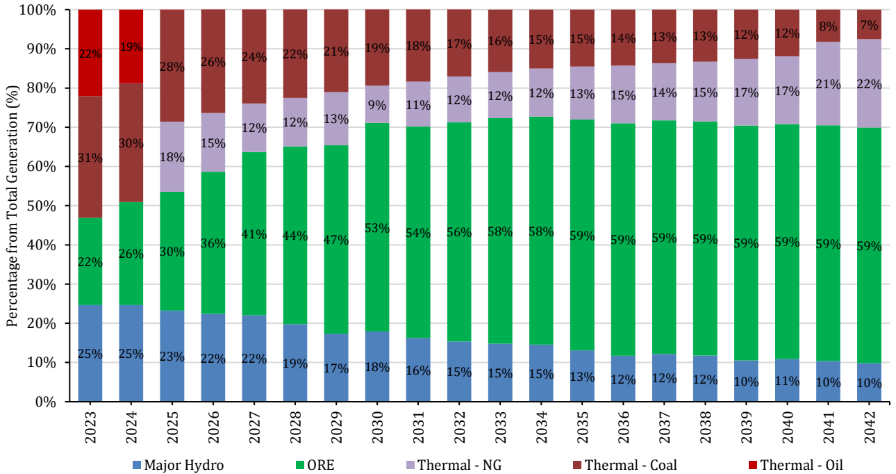
Figure 8.6 – Percentage Share of Energy Mix over Next 20 Years in Base Case
