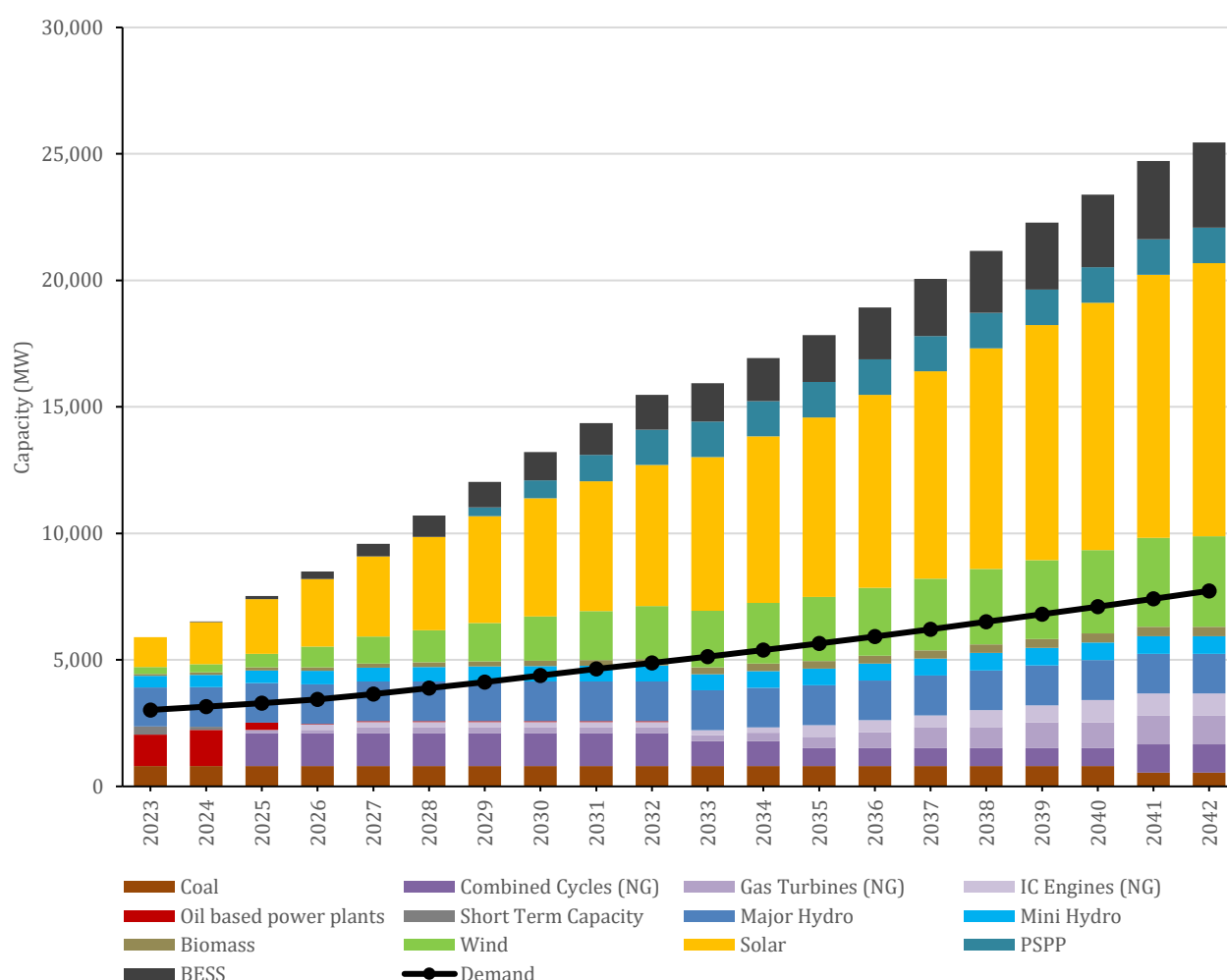
Figure 8.1 –Cumulative Capacity by Plant Type in Base Case
