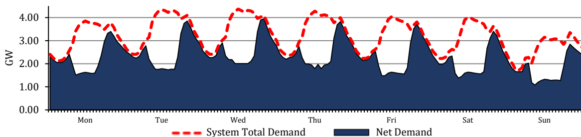
Figure 9.16–Net Demand of Dry Season Week in 2030
