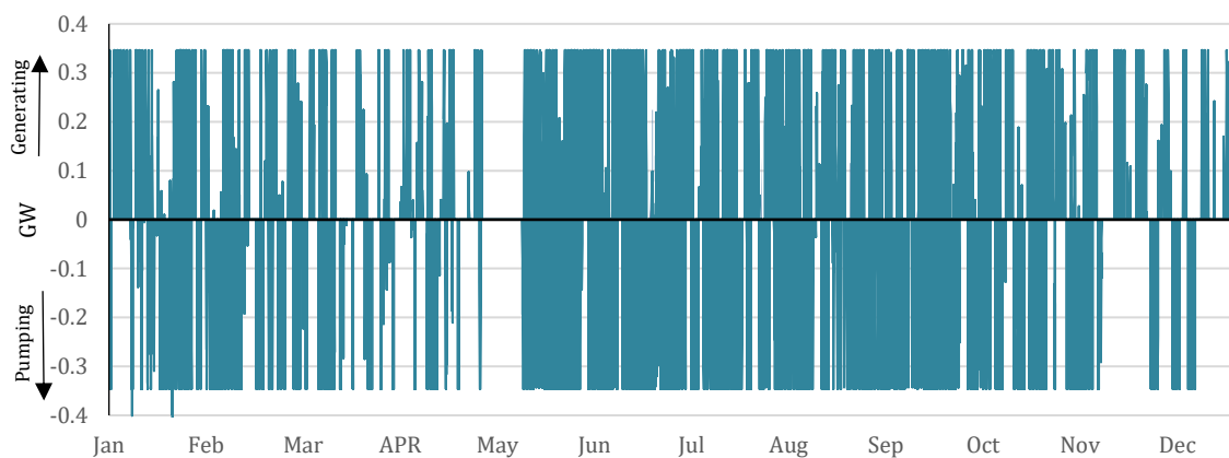
Figure 9.13 – Sample of Pumped Storage Power Plant Operating Pattern of Year 2030
