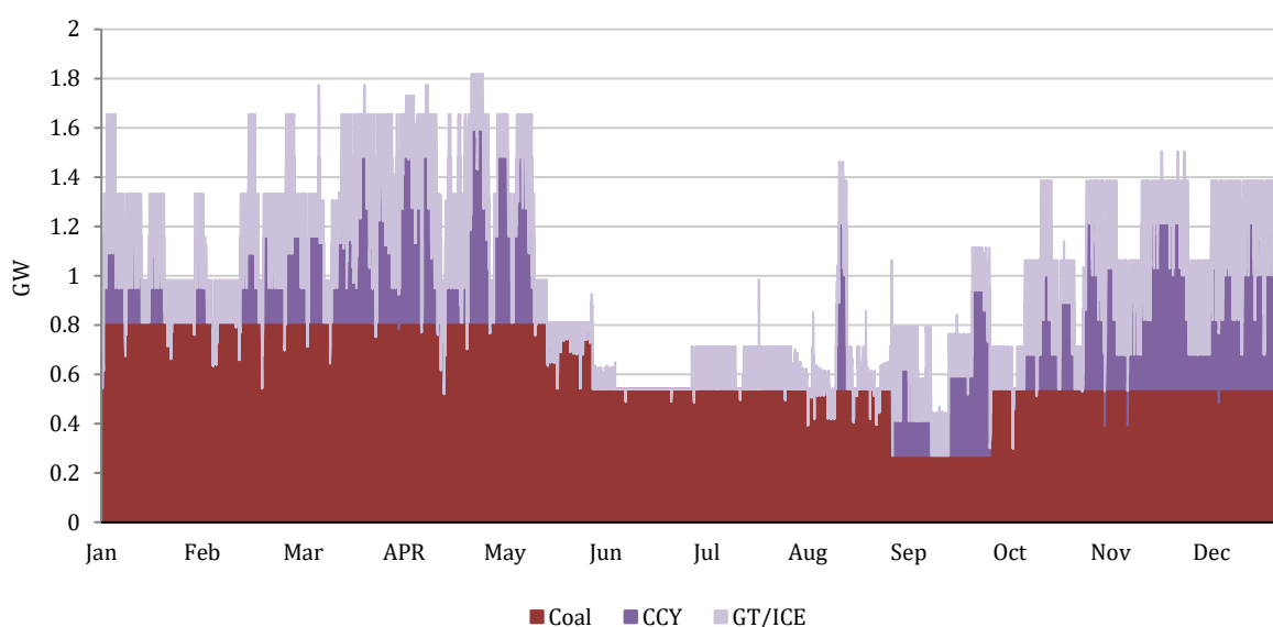
Figure 9.12 – Sample of Thermal Plant Operating Pattern of Year 2030
