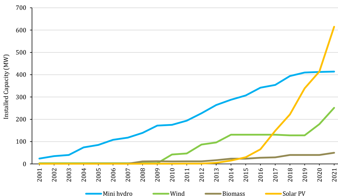
Figure 5.2: Other Renewable Installed Capacity by source 2001-2021
