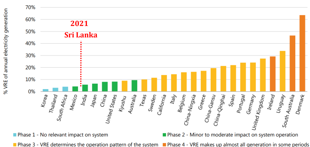
Figure 5.3: Classification of phases based on variable renewable integration challenges
