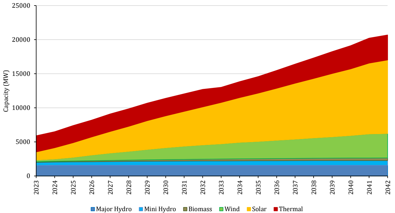
Figure 8.3 – Source wise Capacity Contribution over Next 20 Years
