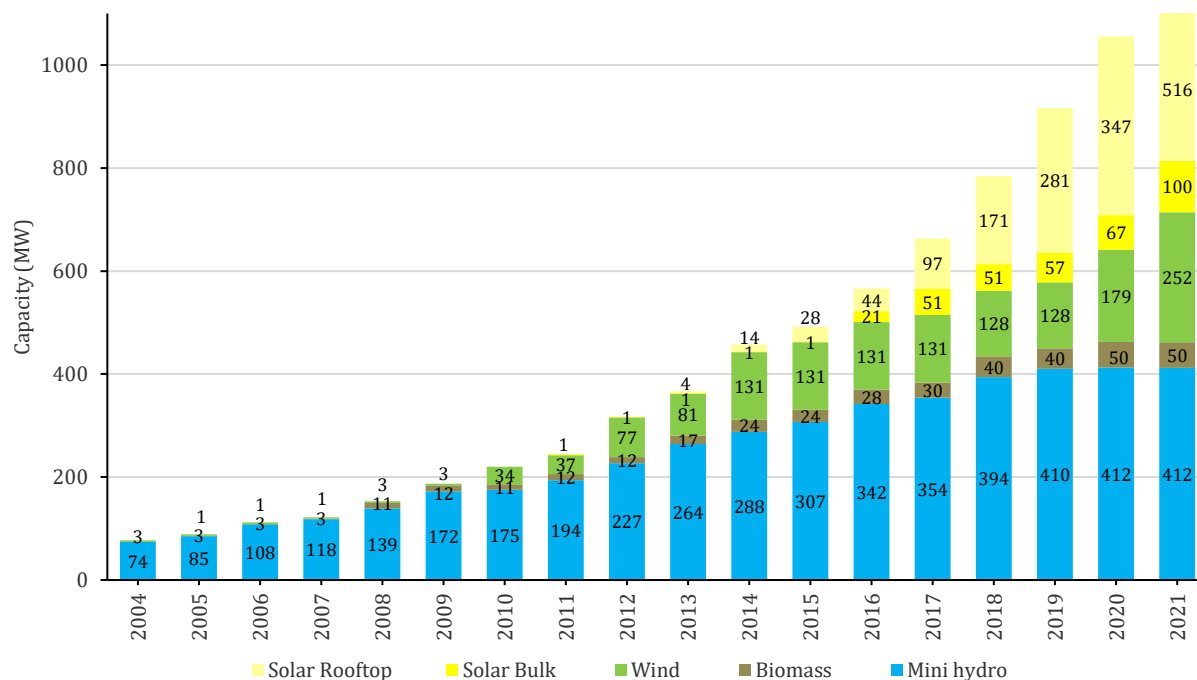
Figure 1.13 – Other Renewable Energy Capacity Development
