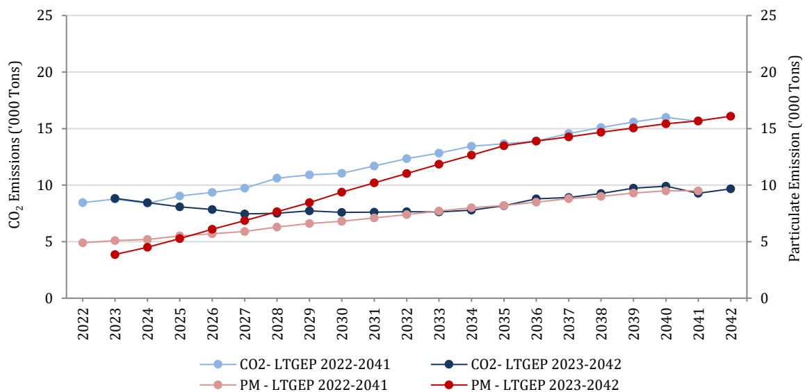
Figure 15.7 - CO 2 and PM Emissions Comparison Between LTGEP 2022-2041 & LTGEP 2023-2042
