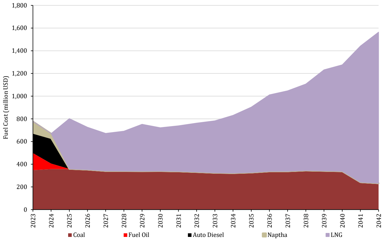
Figure 8.9 - Fuel Cost of Base Case
