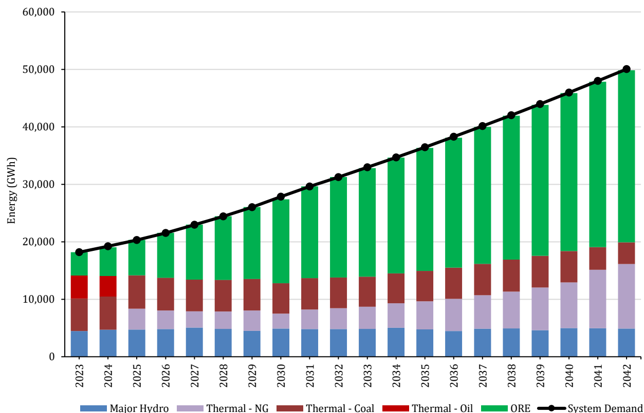
Figure 8.5 – Energy Mix over Next 20 Years in Base Case
