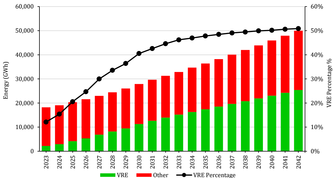
Figure 9.1 – VRE Energy Share in the Base Case
