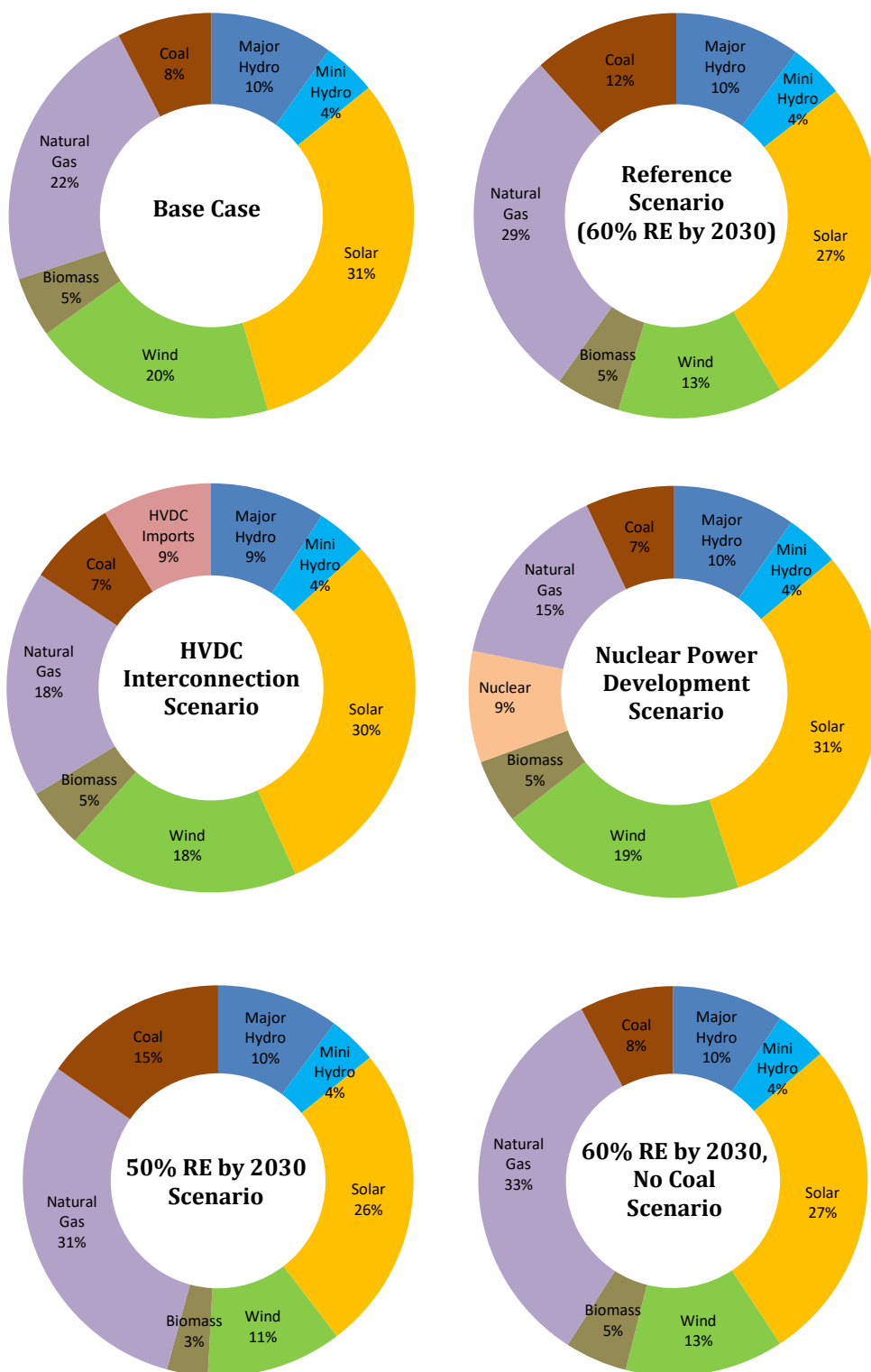
Figure 10.4 –Energy Share Comparison in 2042
