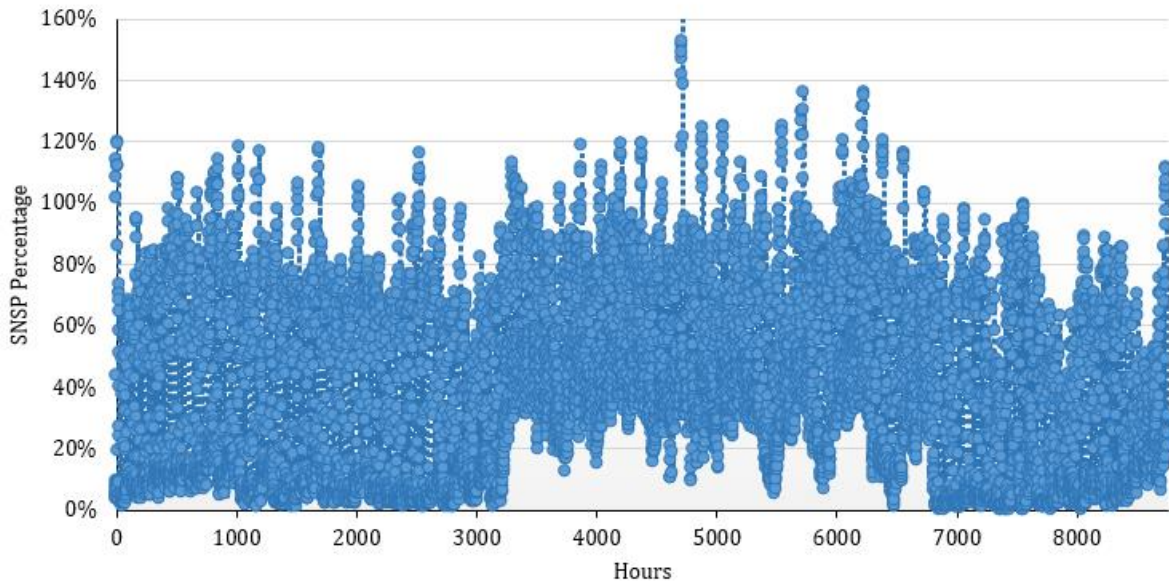
Figure 9.3 – SNSP without Storage & Curtailment in 2030
