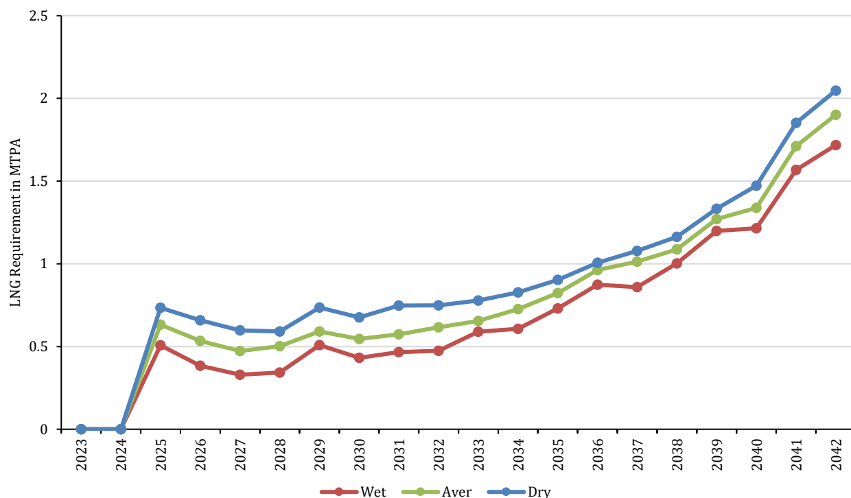
Figure 8.10 - Expected Annual Natural Gas Requirement of the Base Case in Different Hydro Scenarios
