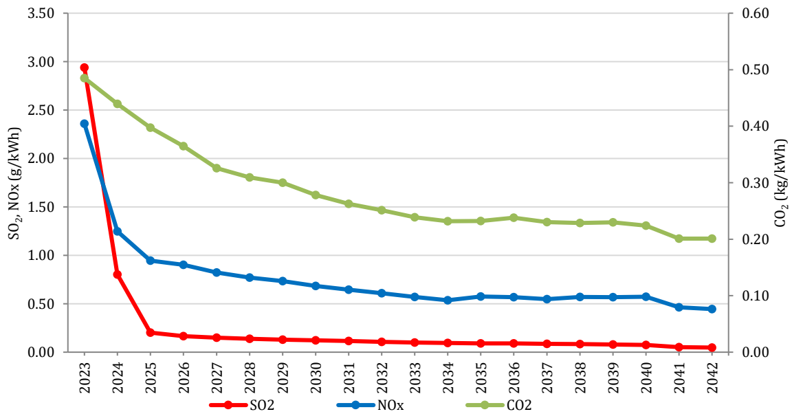
Figure 11.4 – SO 2 , NO x and CO 2 emissions per kWh generated
