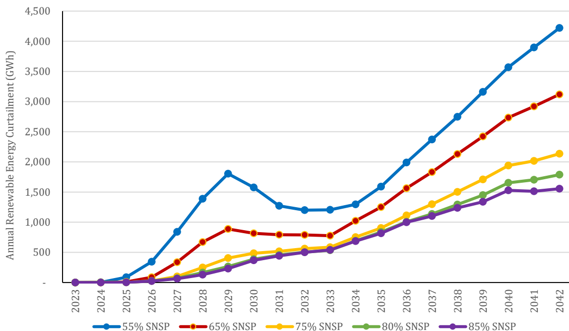
Figure 9.9 – Renewable Energy Curtailments 2023-2042 (varying SNSP)
