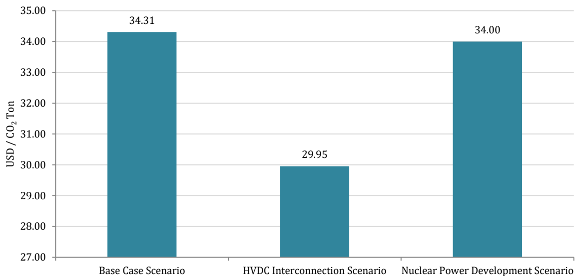
Figure 11.11 – Comparison of Incremental Cost for CO 2 reduction
