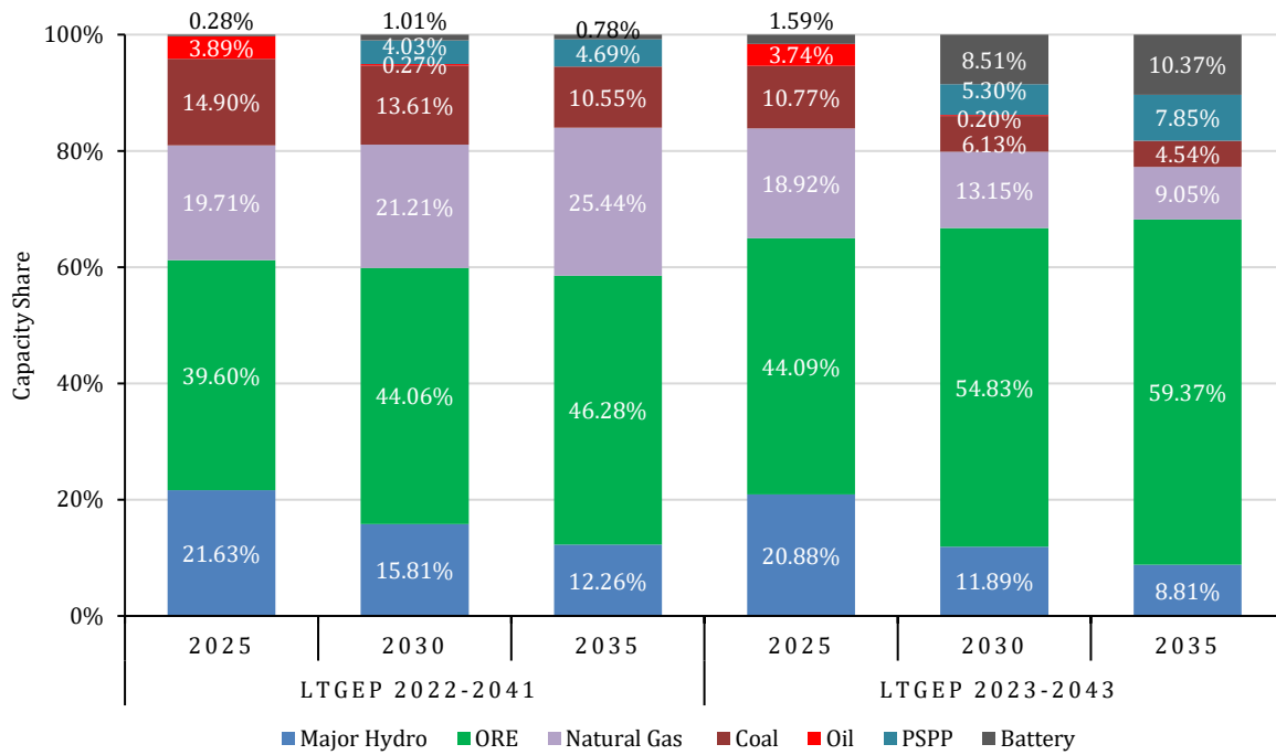
Figure 15.5 – Capacity Share Comparison between LTGEP 2022-2041 & LTGEP 2023-2042
