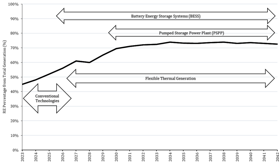
Figure E1 –Achieving 70% RE Target and Proposed Enabling Interventions in Base Case
