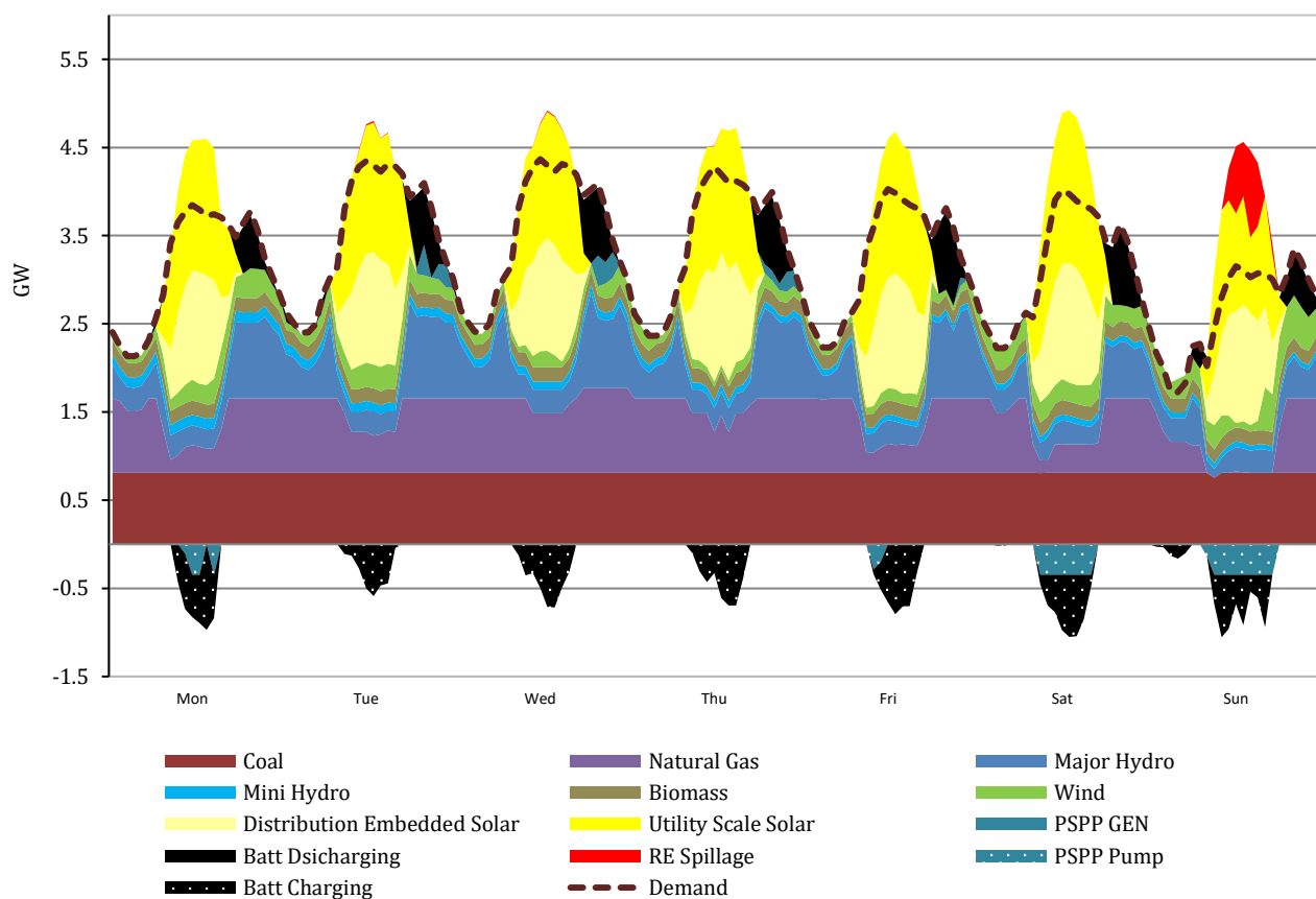
Figure 9.5 – Sample Weekly Dispatch During Dry Season – March 2030
