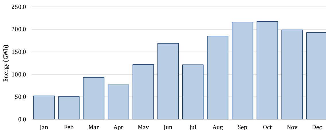
A5.8 Monthly energy production of Mini-hydro resource
