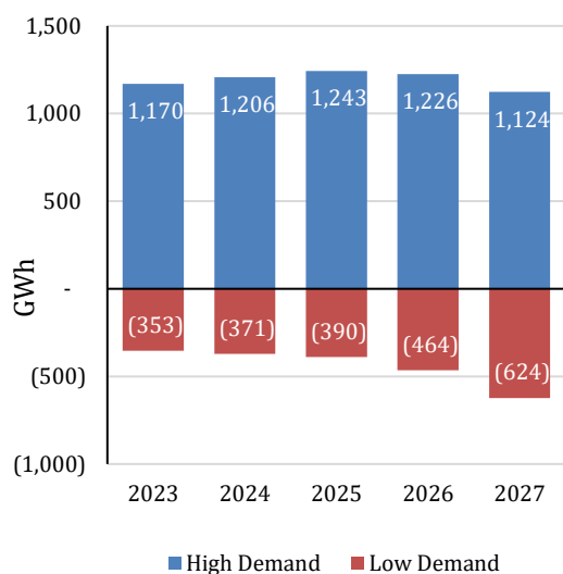
Figure 14.1 –Annual energy demand differences of high and low demand projections relative to base demand forecast
