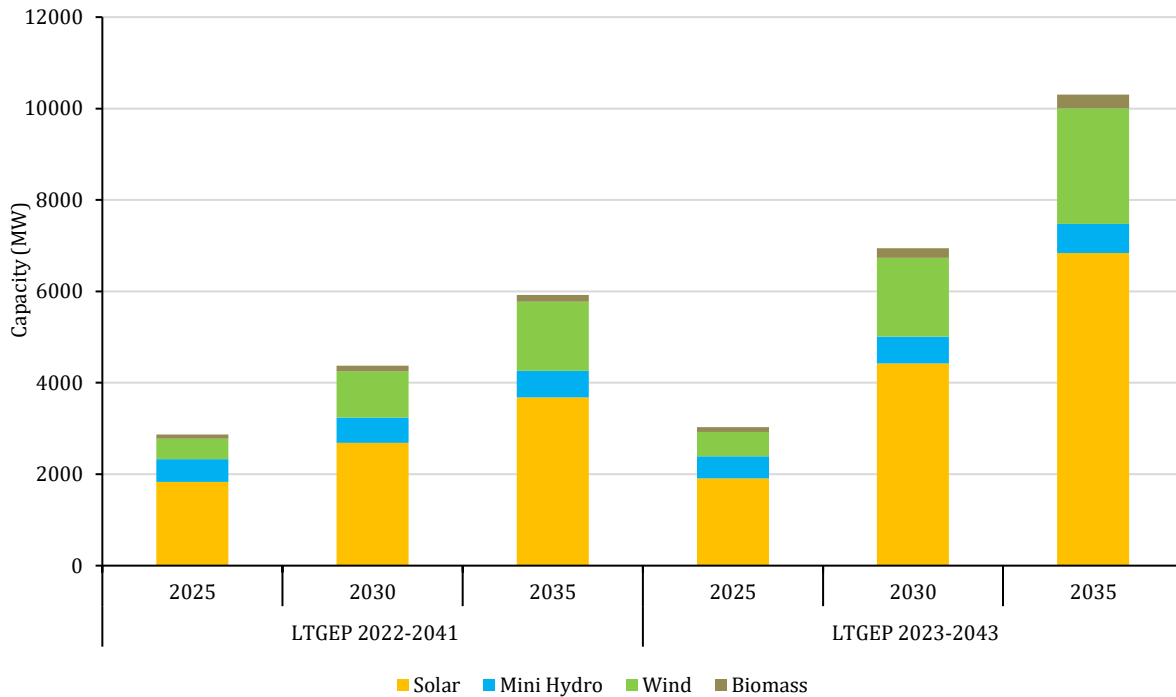
Figure 15.4 – Comparison of ORE Capacities in LTGEP 2022-2041 & LTGEP 2023-2042
