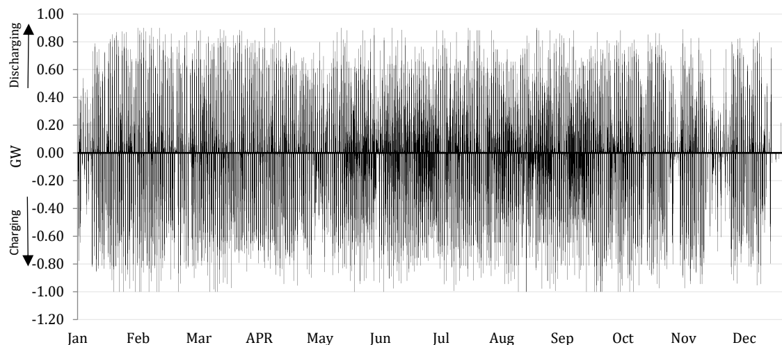
Figure 9.14 – Sample of Battery Energy Storage Plant Operating Pattern of Year 2030
