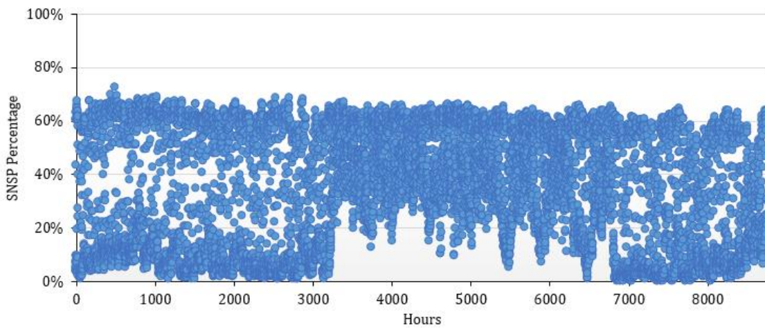
Figure 9.4 – SNSP Constrained with 65% Limit with Storage & Curtailment in 2030
