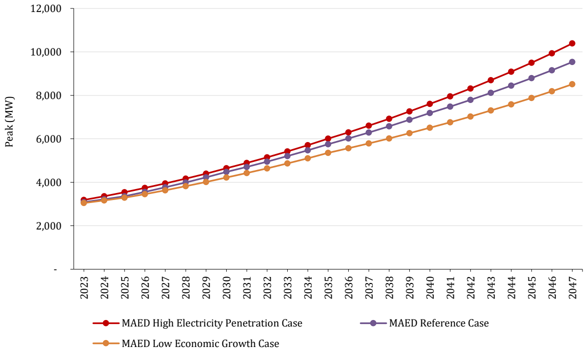
Figure 3.9 - Peak Demand Forecast Comparison - MAED Model
