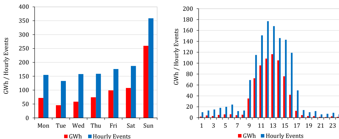
Figure 9.11 - Average Weekly Curtailment Pattern and Average Daily Curtailment of Year 2030
